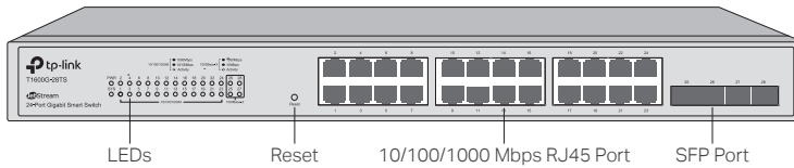
Figure 1-4 Front Panel of T1600G-28TS
