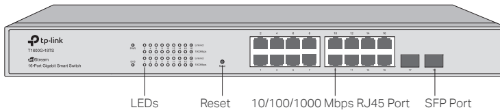
Figure 1-3 Front Panel of T1600G-18TS (TL-SG2216)
