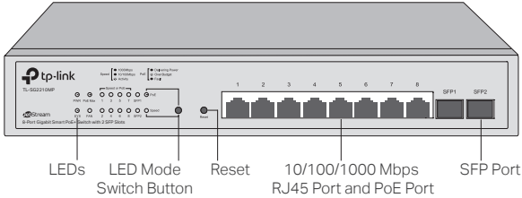
Figure 1-9 Front Panel of TL-SG2210MP
