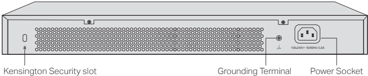
Figure 1-11 Rear Panel
