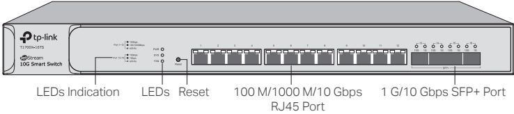
Figure 1-8 Front Panel of T1700X-16TS
