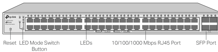
Figure 1-6 Front Panel of T1600G-52PS (TL-SG2452P)
