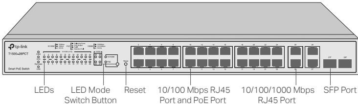
Figure 1-2 Front Panel of T1500-28PCT (TL-SL2428P)
