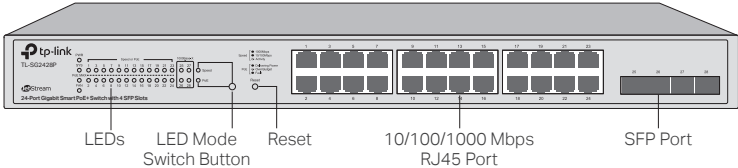
Figure 1-10 Front Panel of TL-SG2428P
