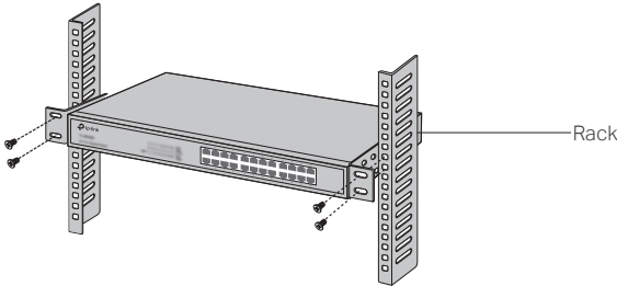
Figure 2-3 Rack Installation
